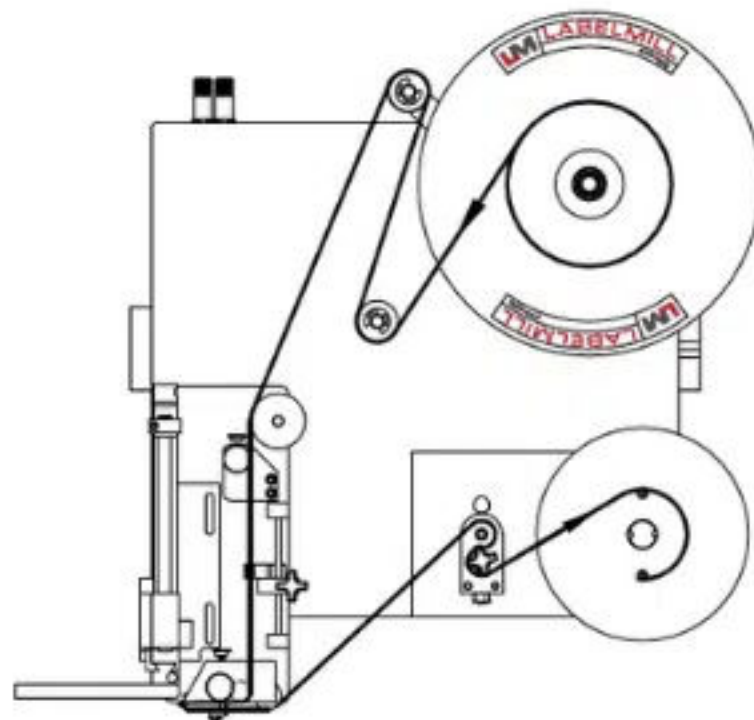
Left Hand Label Applicator Horizontal Feed Right to Left Webbing
