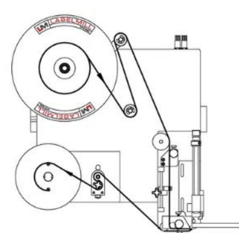
Right Hand Label Applicator Horizontal Feed Left to Right Webbing
